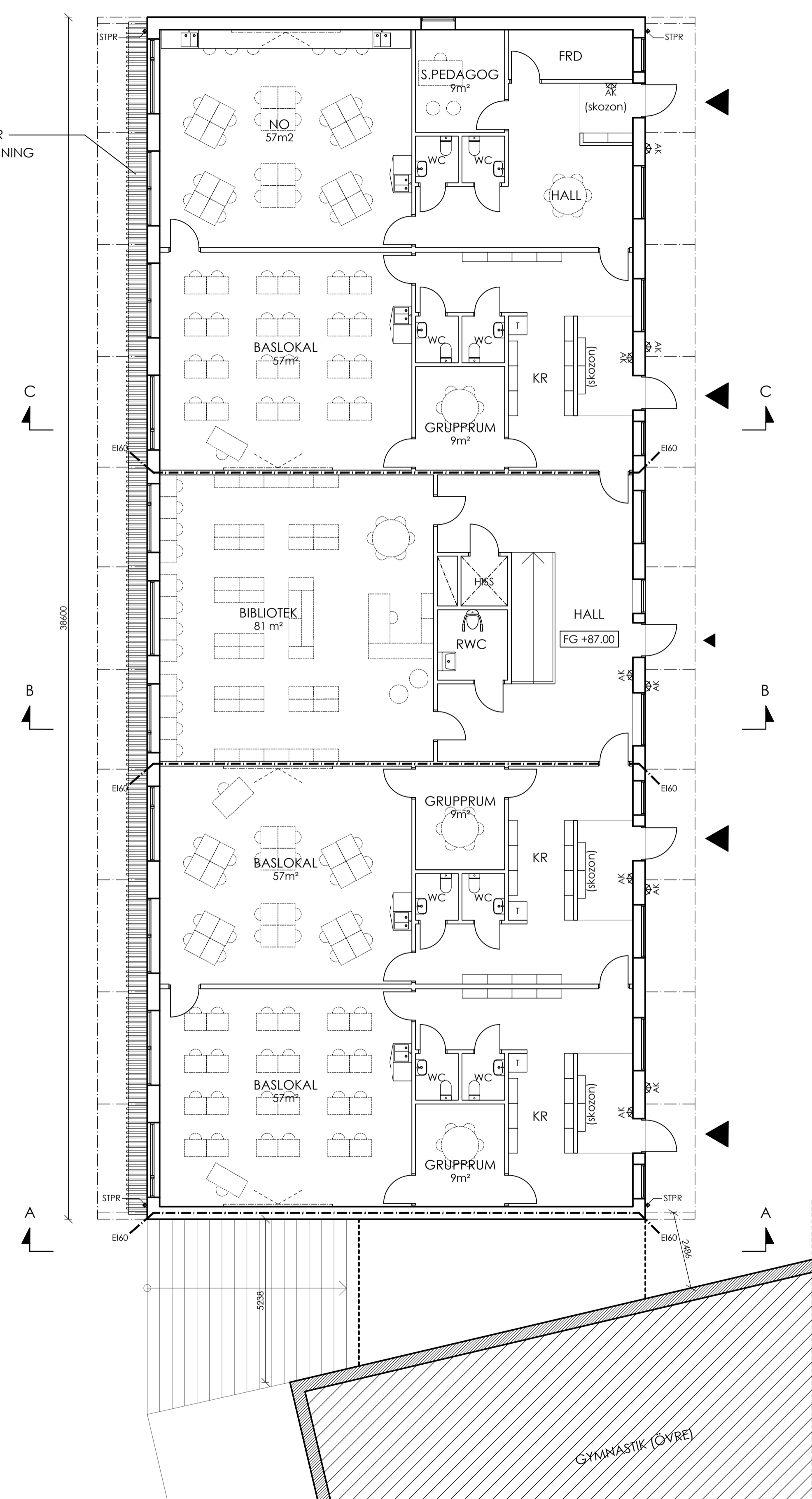
PLAN 10 (GÅRDSPLAN) SKALA 1:100 (A1)
